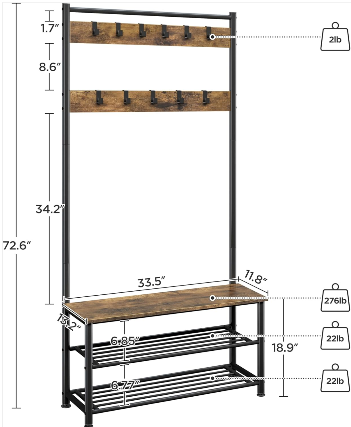
Figure 4.1: Product dimensions and weight capacities.
