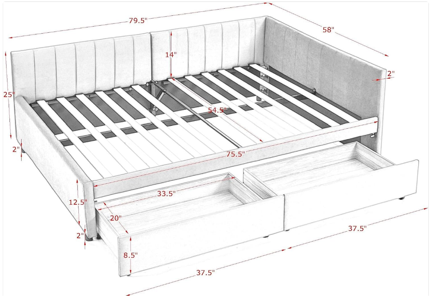
Figure 3.3.1: KEIKI Daybed demonstrating open storage drawers.
