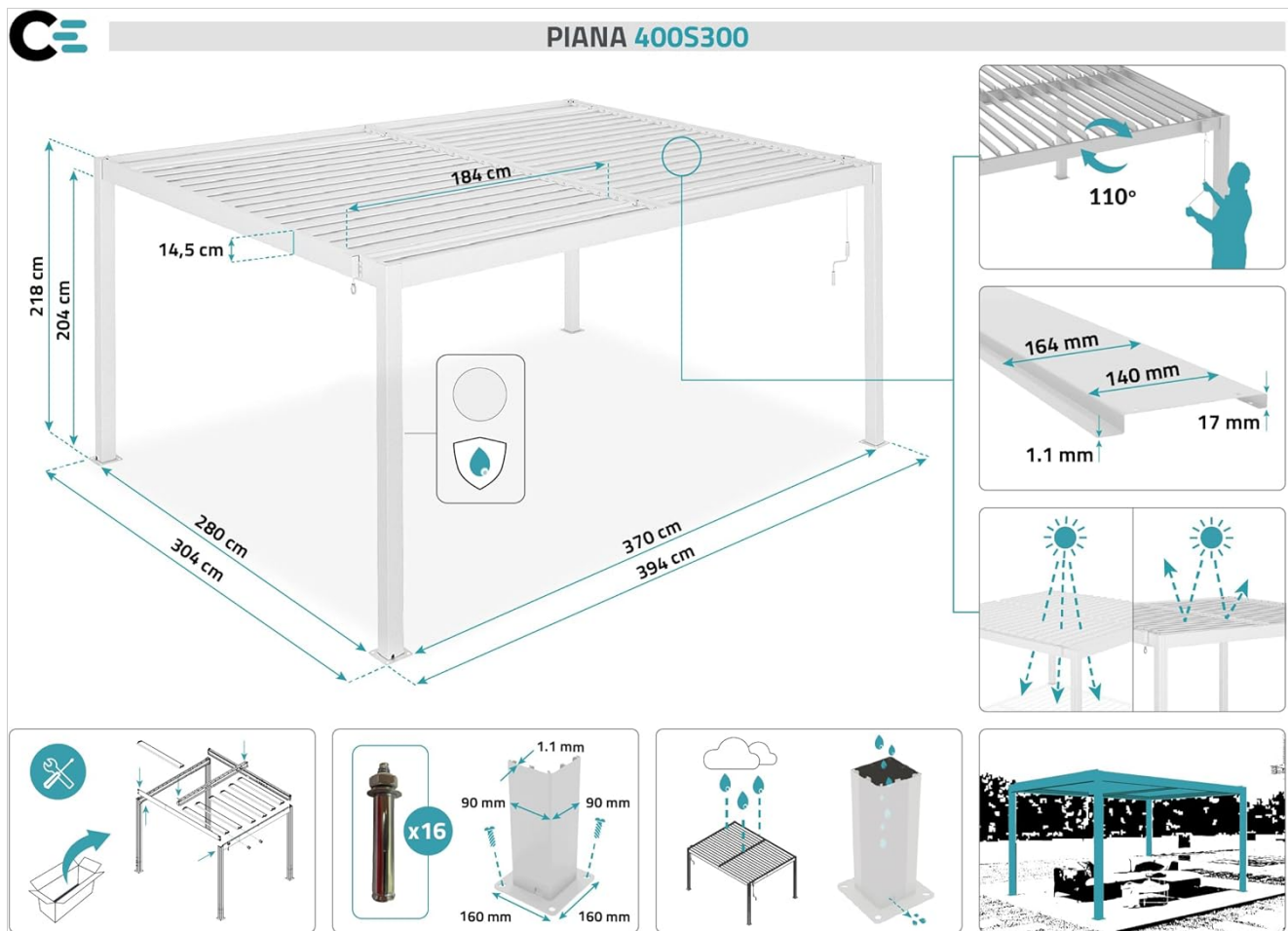
Image: Detailed dimensions and features of the Cazeboo Piana Bioclimatic Pergola. This diagram illustrates the overall dimensions of the pergola (Length, Width, Height), including specific measurements for the louvers and posts. It also highlights the 110-degree adjustability of the louvers and the integrated water drainage system.
