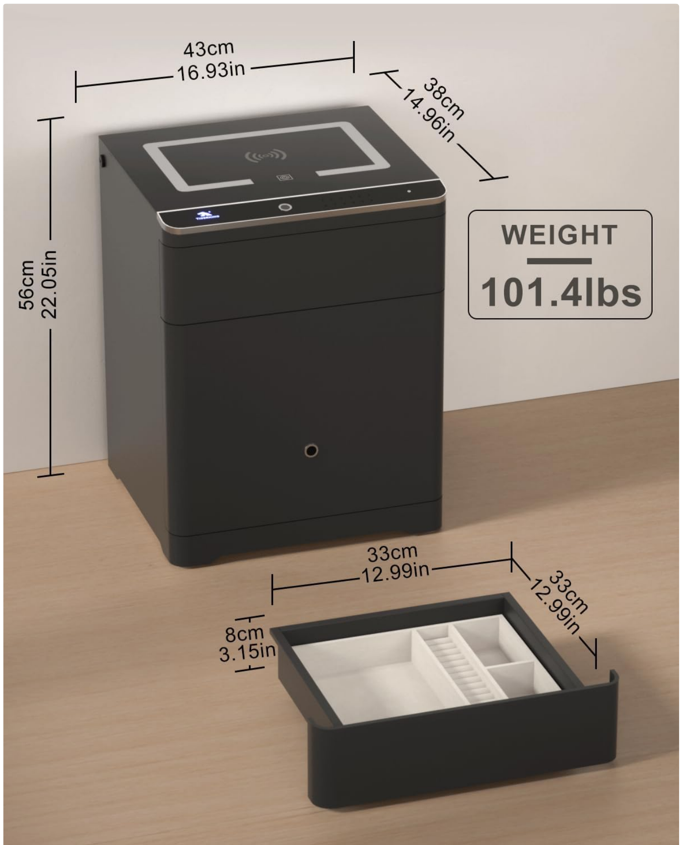
Figure 2.1: Detailed dimensions and weight of the safe.
