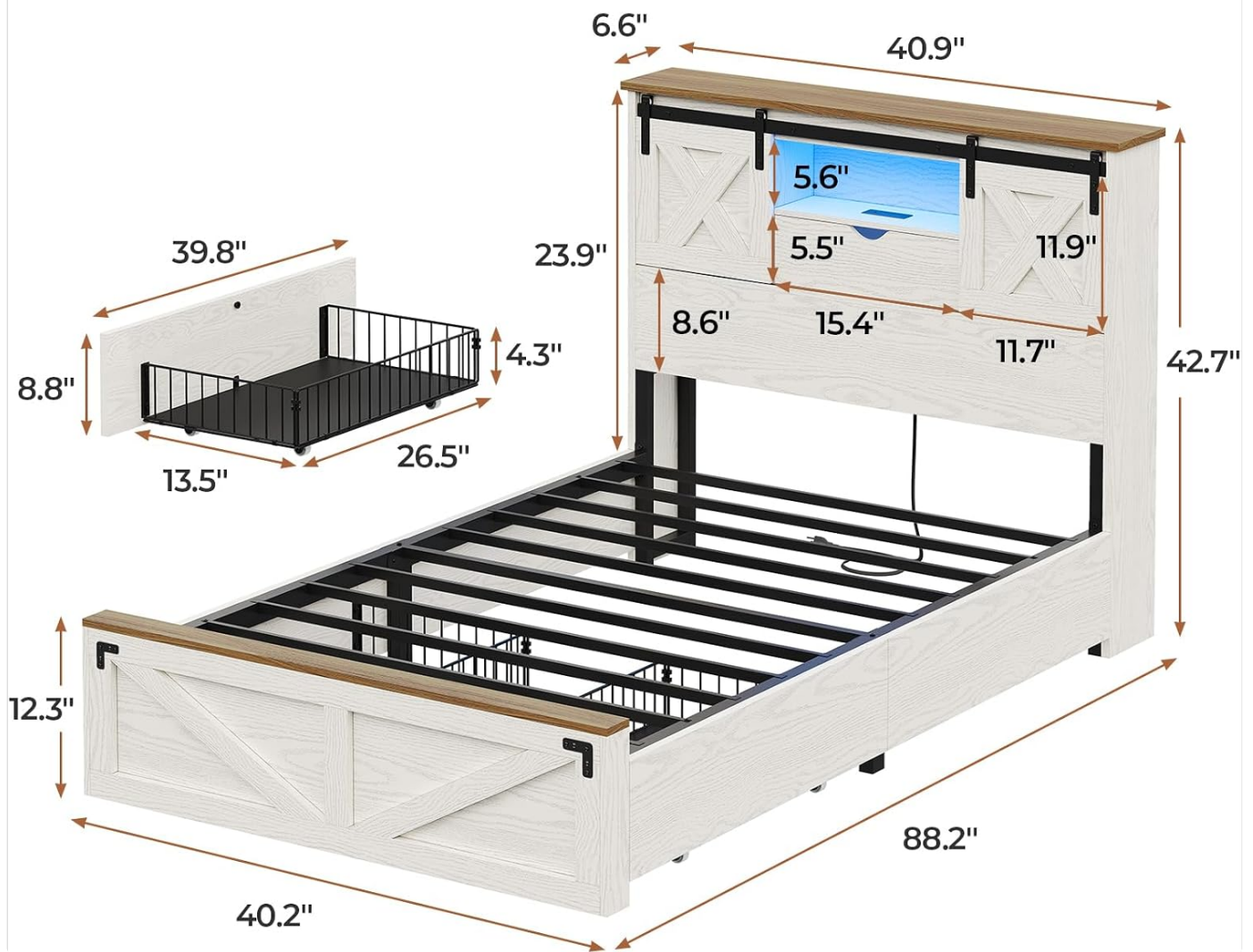
Figure 5: Farmhouse Storage Headboard. This image provides a clear view of the headboard's storage capabilities, including the sliding barn doors, rustic accent decor, and a storage cubby with a door, highlighting its functional design.
