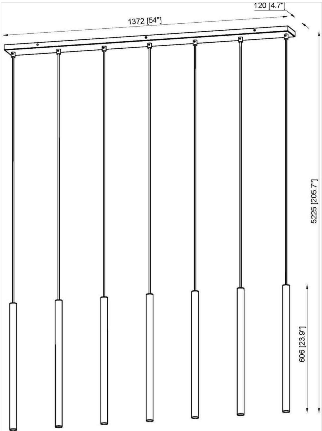
Figure 1: Dimensional drawing of the chandelier, illustrating its 54-inch length, 4.75-inch width, and 23.75-inch height.
