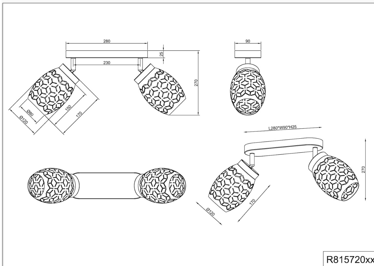
Image 4.2: Technical drawing showing detailed measurements and angles for installation.
