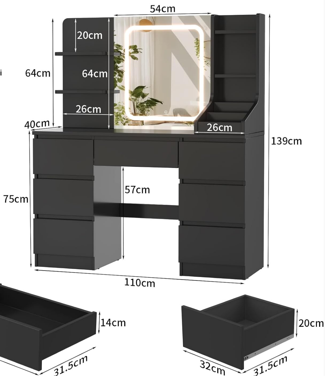
Image 4.1: Detailed dimensions of the TRIUMPHKEY DT-0513 Dressing Table.
