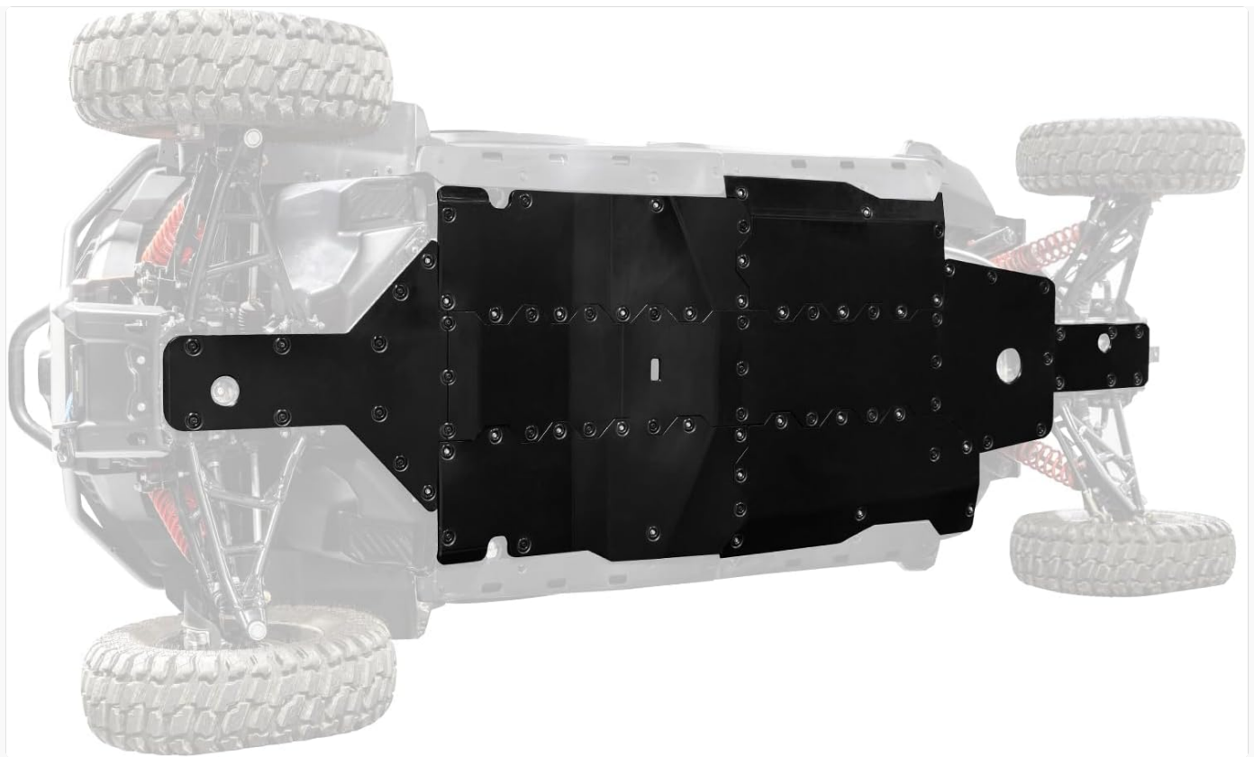
Figure 1: The SuperATV Full Skid Plate fully installed on the underside of a CFMOTO ZForce 950 Sport 4. This image highlights the extensive coverage provided by the multi-panel system, secured with numerous countersunk bolts.
