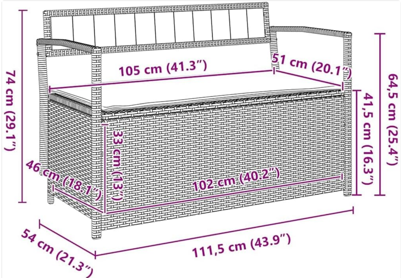
Image: Technical drawing illustrating the precise dimensions of the vidaXL Patio Storage Bench, including overall width, depth, height, and internal storage measurements.
