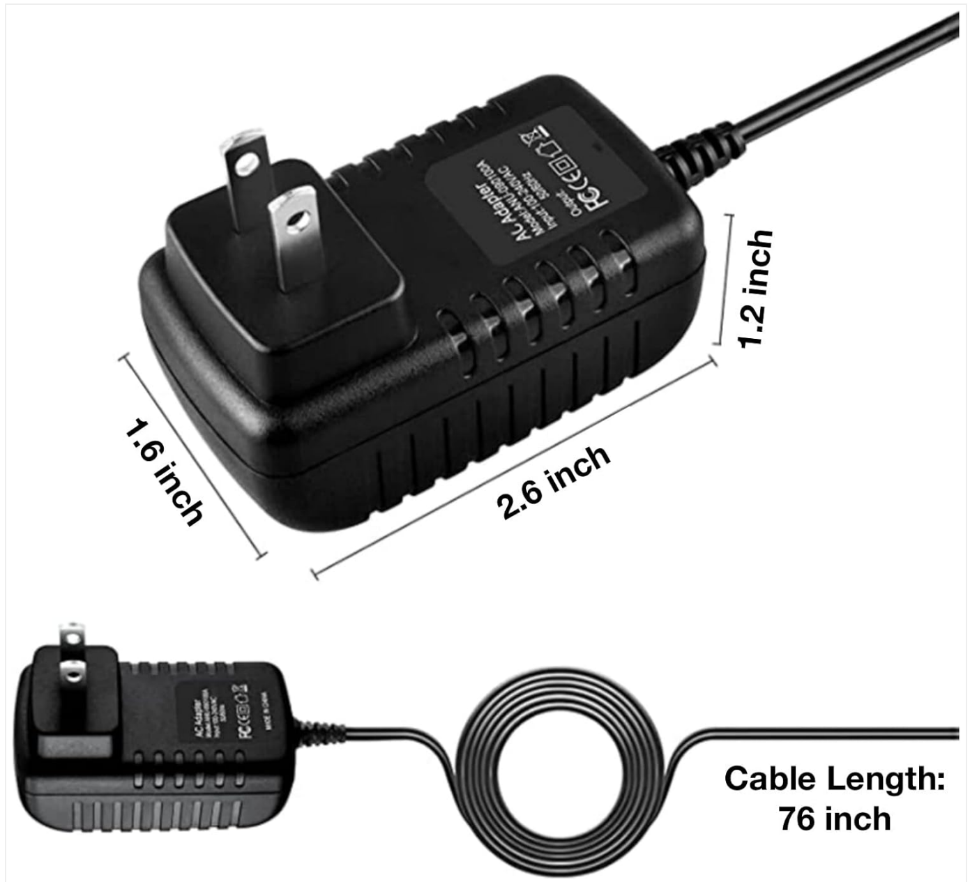
Image 3.2: This image illustrates the physical dimensions of the adapter body (approximately 2.6 inches long, 1.6 inches wide, and 1.2 inches high) and the total cable length (approximately 76 inches).
