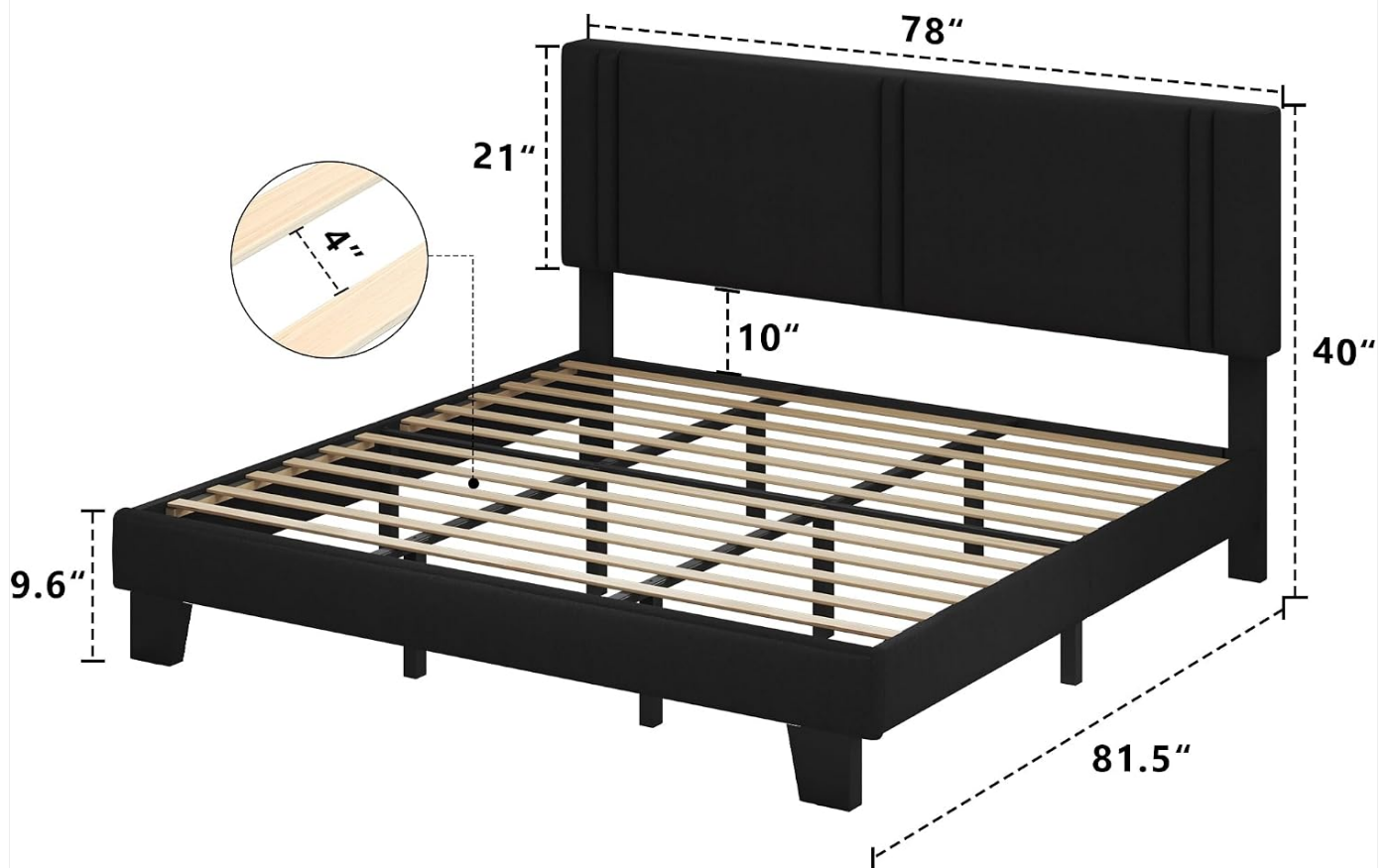
Figure 4: Dimensions and Capacity. This diagram provides the overall dimensions of the King size bed frame (81.5"L x 78"W x 40"H), its maximum weight capacity of 800 lbs, and the recommended mattress thickness of 8-12 inches.
