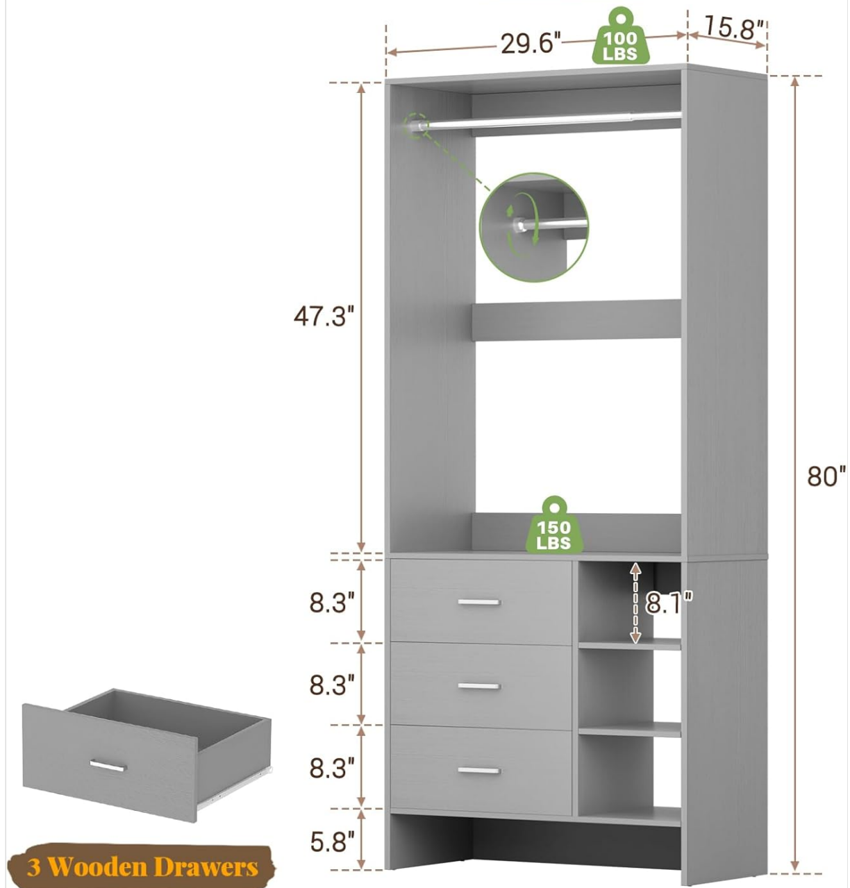
Figure 8.1: Visual representation of the Aheaplus Closet System's dimensions and weight capacities for various sections.
