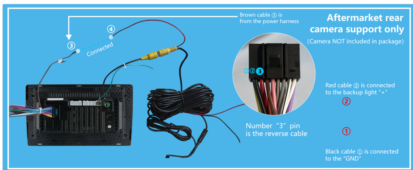
Image: Aftermarket rear camera wiring diagram, detailing connections for power, ground, and reverse signal.
