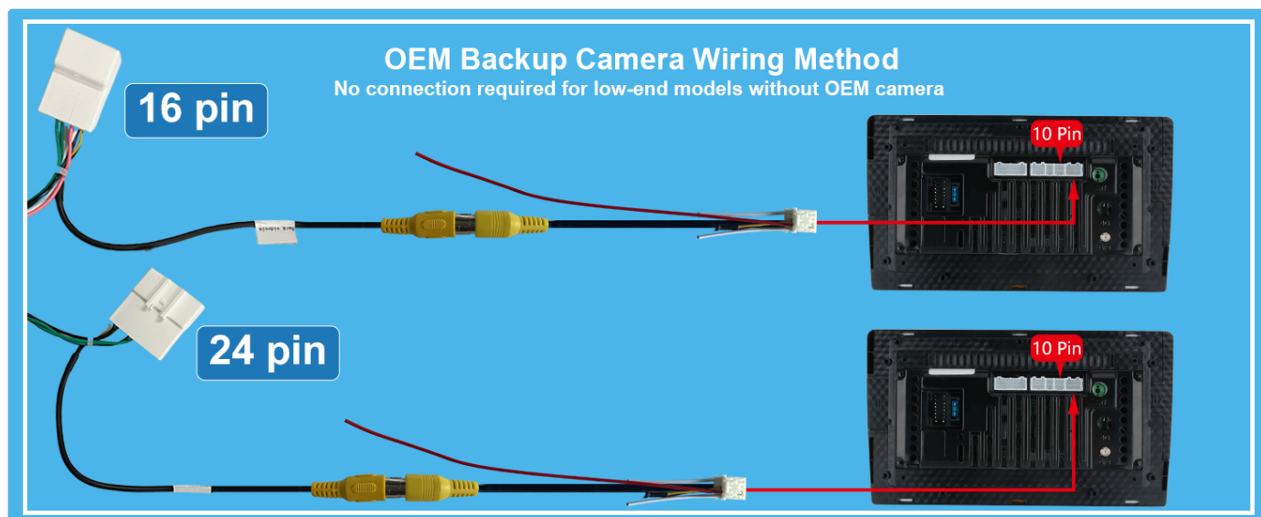
Image: OEM backup camera wiring instructions for 16-pin and 24-pin connectors, showing connection points to the car stereo.
