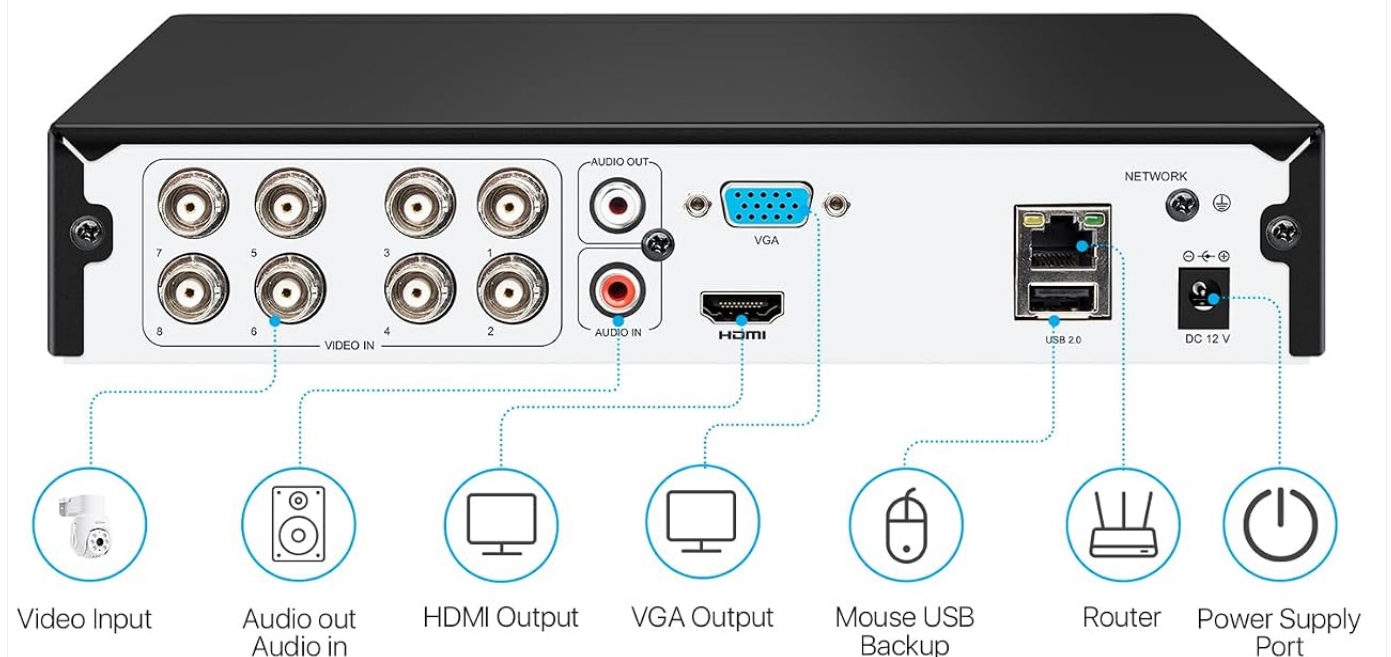
Image: Rear panel of the ZOSI DVR with labeled ports for video input, audio out/in, HDMI, VGA, USB, network, and power supply.
