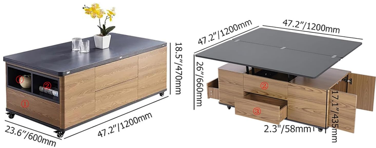
OPEN SHELF ①&② INNER DIMENSION
