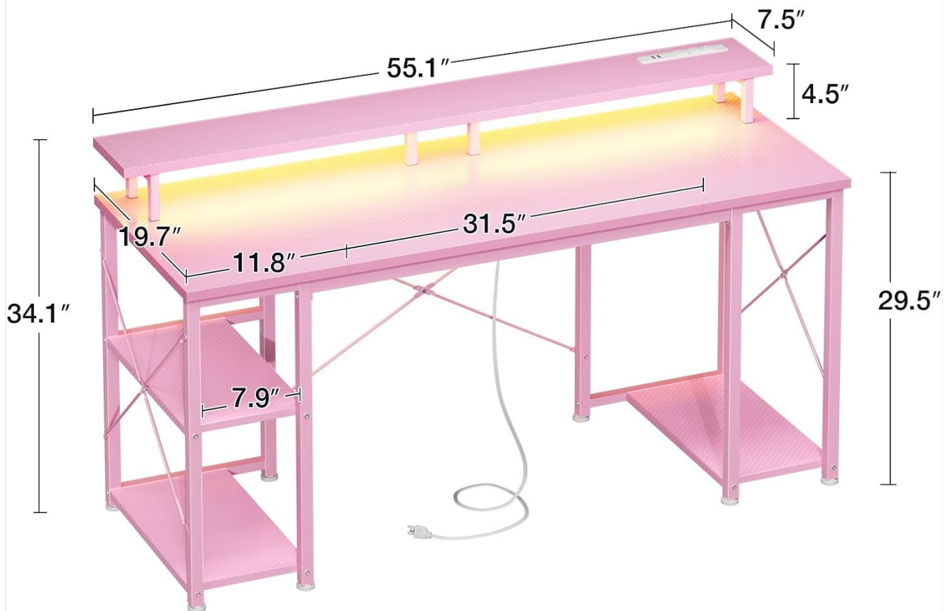
Image: Detailed diagram illustrating all components and their respective dimensions for the ODK 55-inch Gaming Desk.
