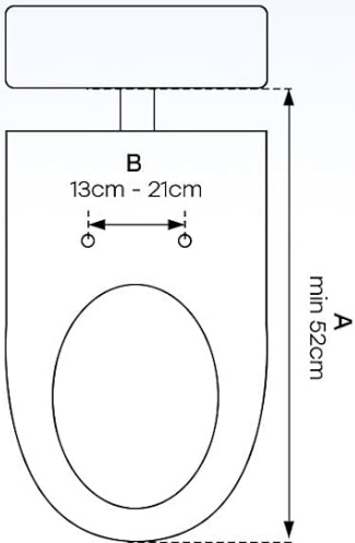
Image: A diagram illustrating the required dimensions for both wall-hung and floor-mounted toilets to ensure compatibility with the bidet seat. Key measurements for length, width, and bolt spacing are shown.
