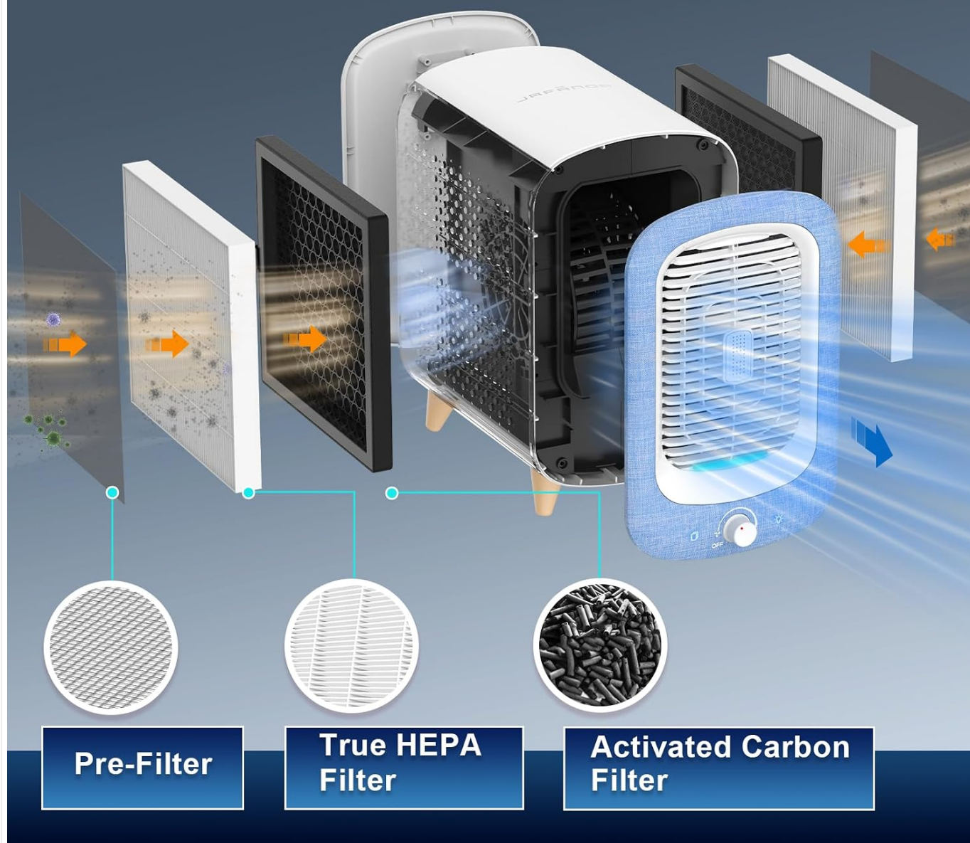
Image: A detailed diagram showing the airflow and the three stages of filtration (Pre-Filter, True HEPA Filter, Activated Carbon Filter) within the Jafanda JF180 air purifier.
