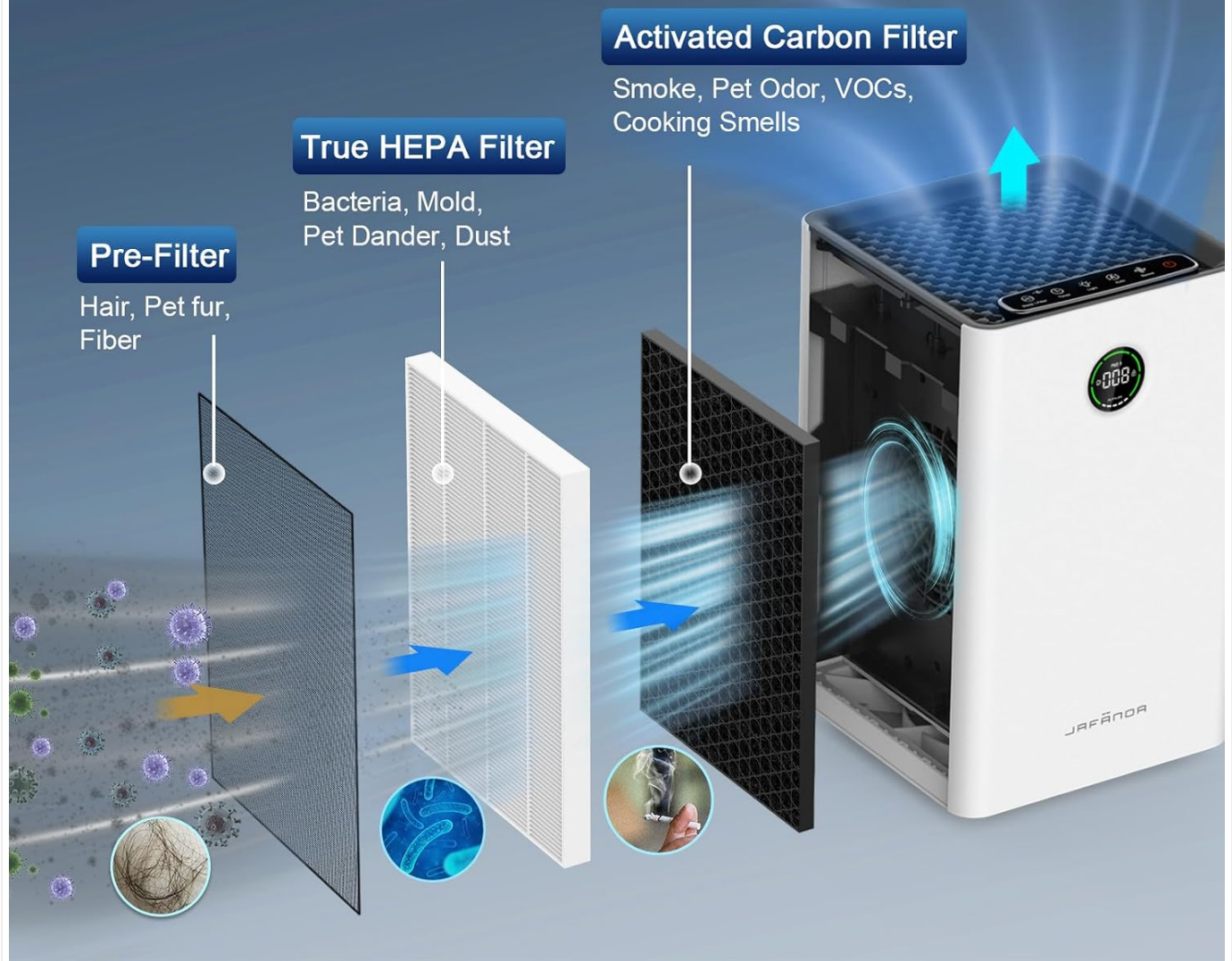
Image: A detailed diagram showing the airflow and the three stages of filtration (Pre-Filter, True HEPA Filter, Activated Carbon Filter) within the Jafanda JF260 air purifier.
