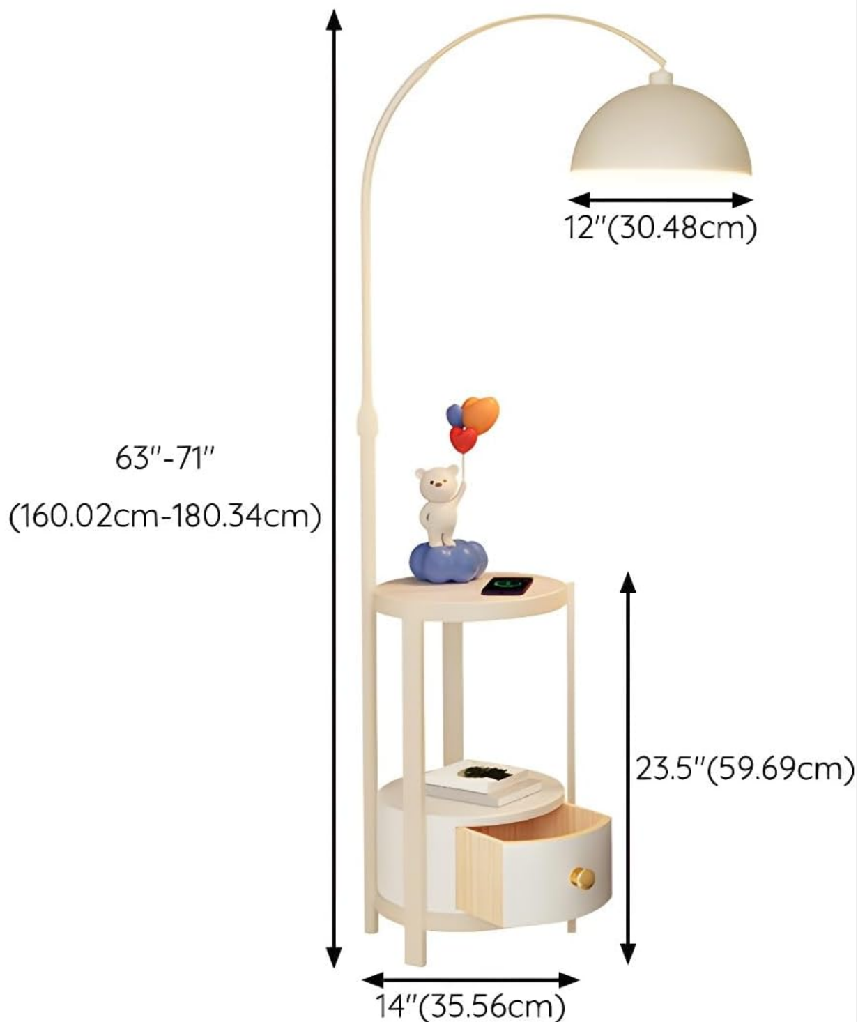
Image 4.1: Dimensional diagram of the lamp, illustrating its adjustable height (63"-71"), shade width (12"), and shelf width (14").
