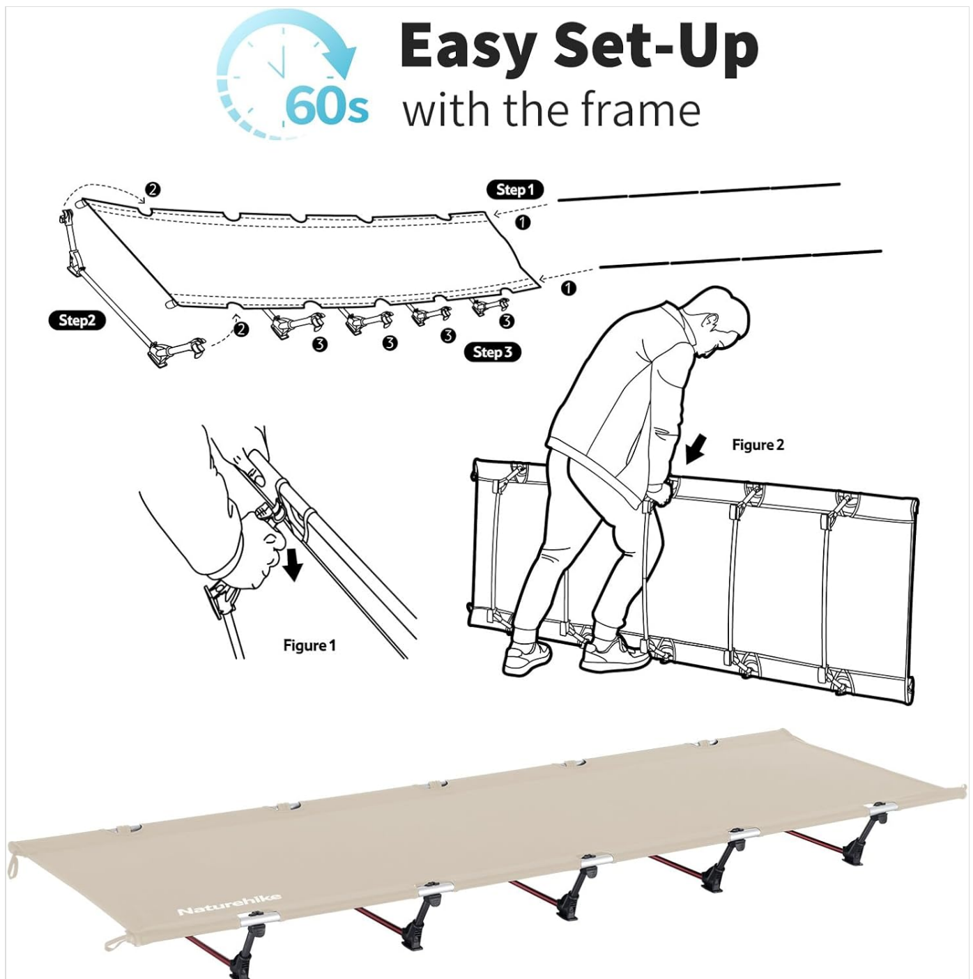
Figure 1: Visual guide for cot frame assembly. Insert poles into sleeves and attach leg supports.
