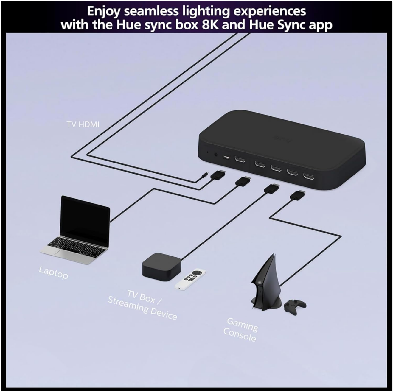
Image: Connection diagram for the Philips Hue Play HDMI Sync Box 8K.
