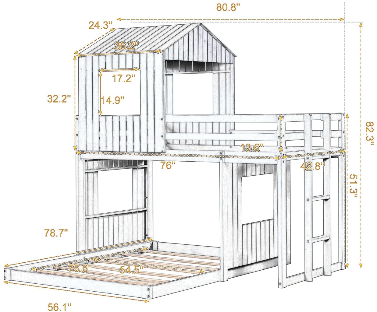
Image 2: Technical drawing illustrating the precise dimensions of the bunk bed, including length, width, and height for both the overall structure and individual components.
