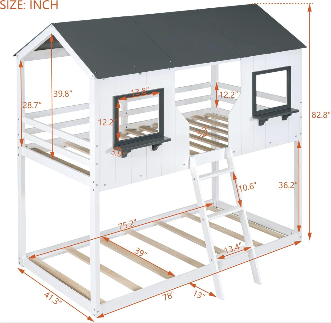
Image 8.1: Technical drawing illustrating the precise dimensions of the bunk bed, including overall length, width, height, and internal measurements for each bunk.
