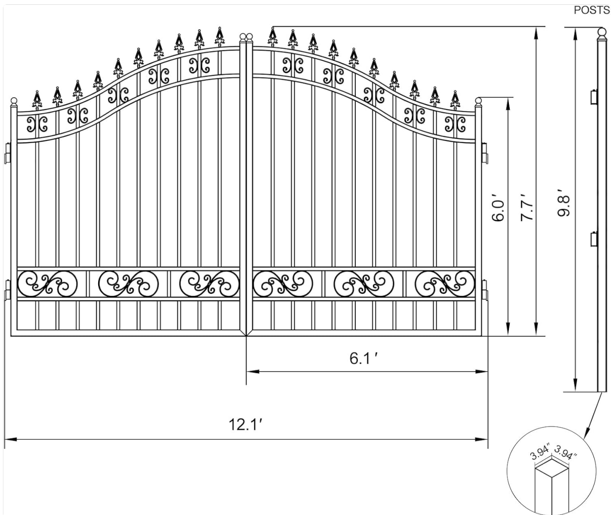
Figure 4.1: Gate and Post Dimensions.
