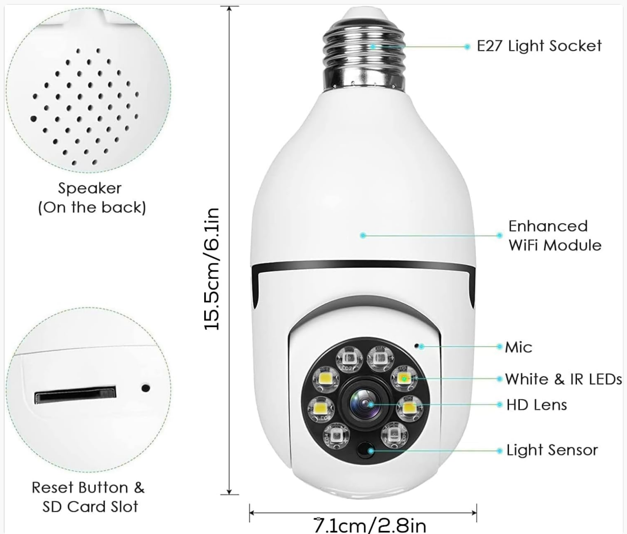
Figure 4.1: QAMY Light Bulb Security Camera Components and Dimensions.
