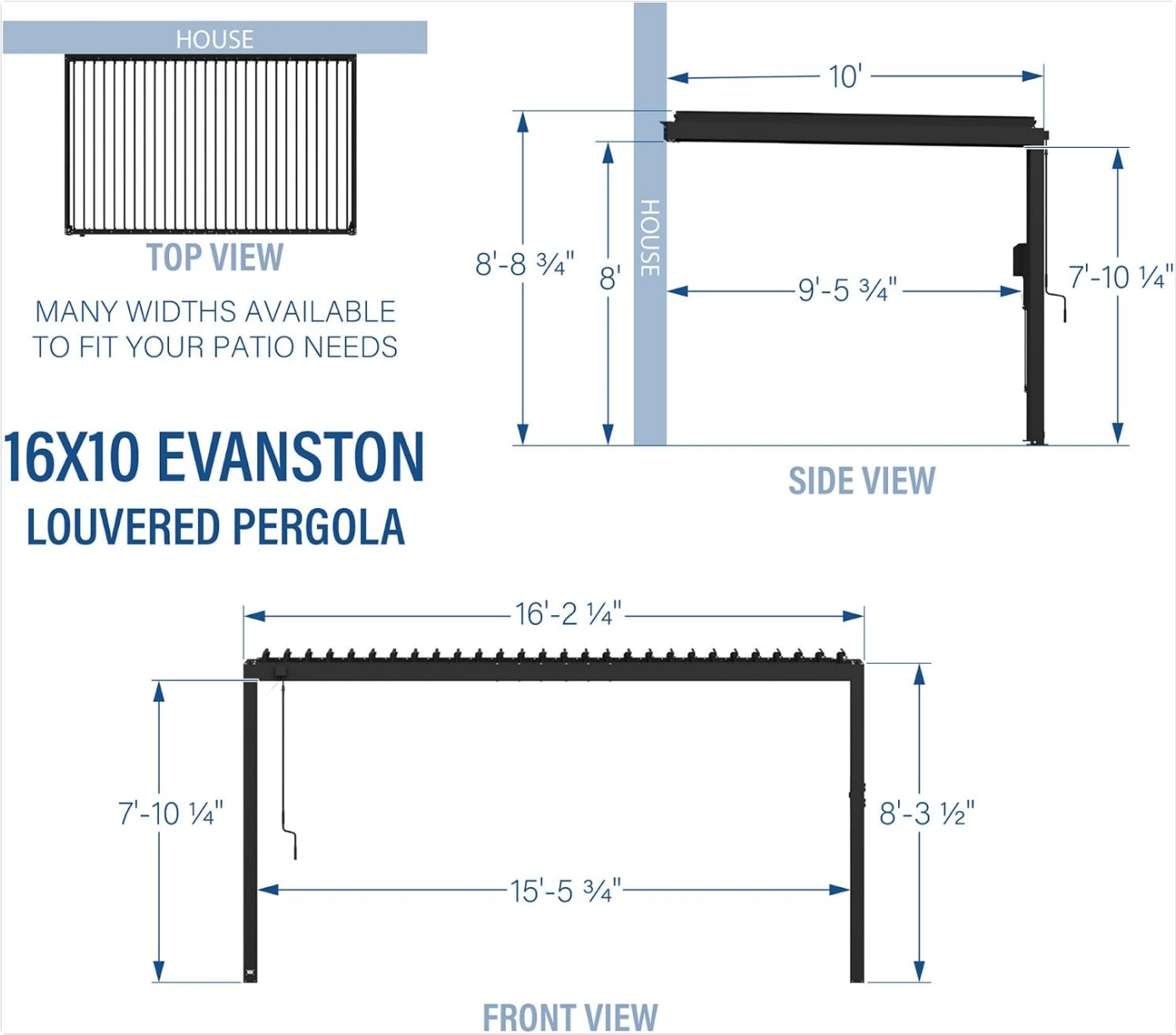
Figure 3: Dimensional diagram for the 16x10 Evanston Wall-Mounted Louvered Pergola.
