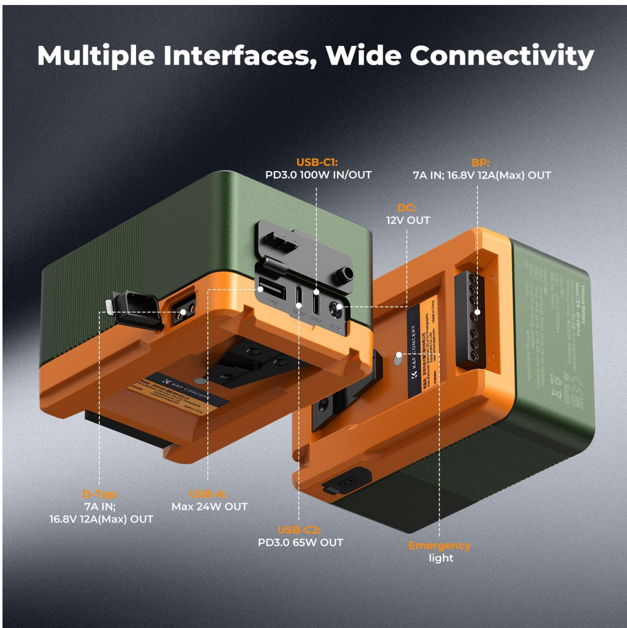
Image: Detailed diagram highlighting the various input and output ports on the K&F CONCEPT V-Mount Battery.
