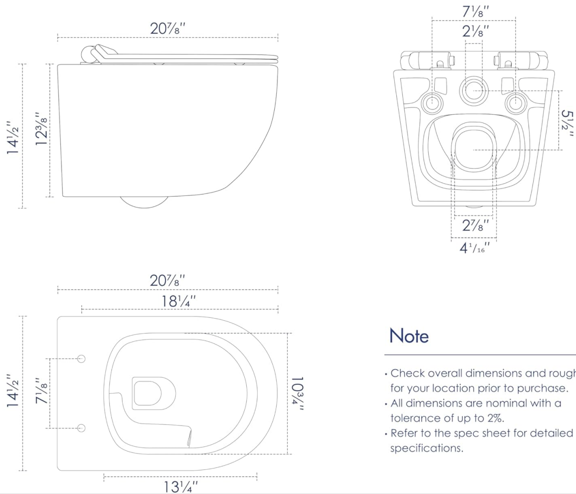
Figure 3: Technical Data for ERI-WT425. Refer to the spec sheet for detailed specifications.
