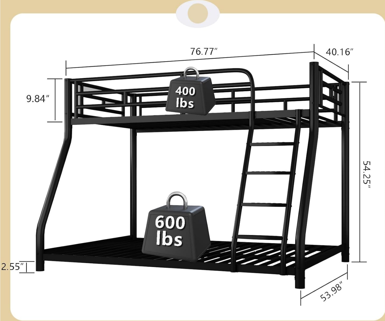
Image: Detailed dimensions and weight limits for the KAIFAM bunk bed.
