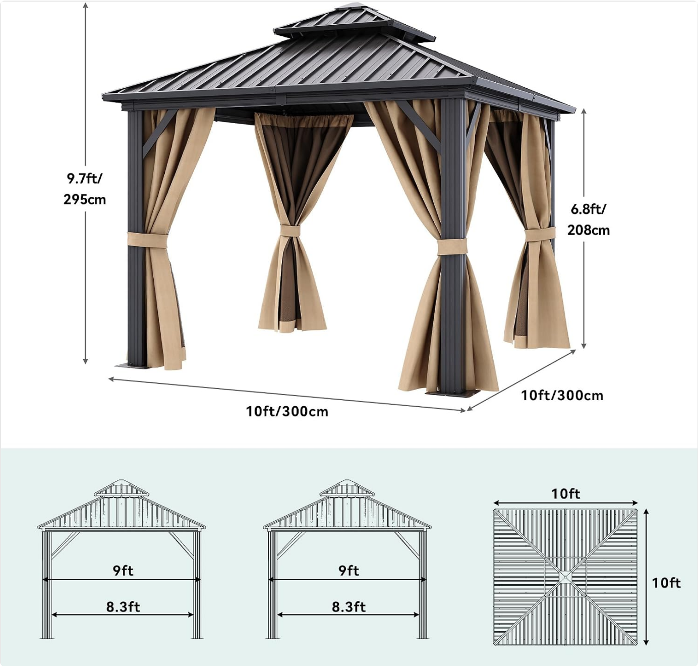
Figure 3: Gazebo dimensions for planning and assembly.
