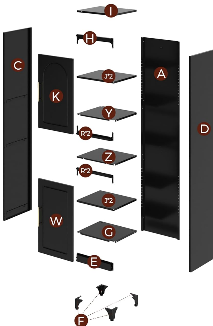
Figure 3.1: Exploded diagram showing all individual components of the cabinet, labeled with letters for easy identification during assembly. This includes side panels, shelves, doors, handles, and adjustable feet.
