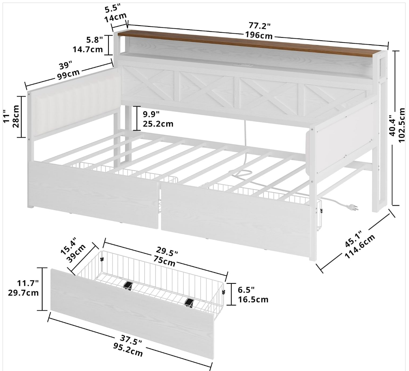
Image: Detailed diagram illustrating the full dimensions of the IRONCK Twin Size Daybed, including length, width, and height measurements.
