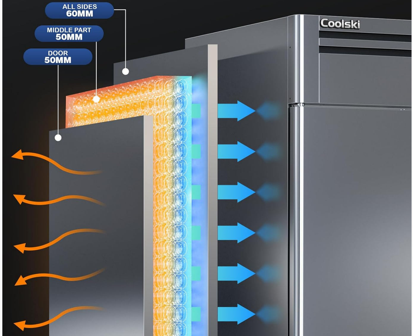
Image 4: Cross-section view demonstrating the high-quality insulation (60mm for all sides, 50mm for middle part and door) for long lifespan and easy cleaning.
