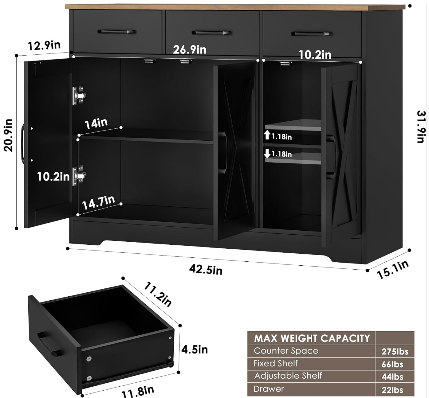
Figure 4: Detailed dimensions and maximum weight capacity.
