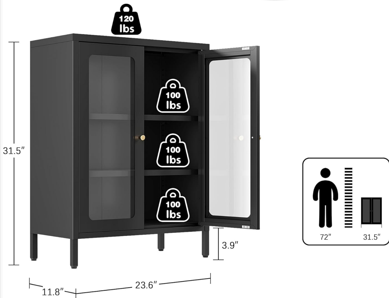
Figure 4: Product Dimensions and Weight Capacities
