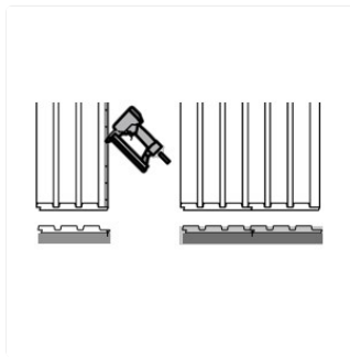
Image: Illustration of the shiplap interlocking mechanism, demonstrating how panels connect for a flush installation.
