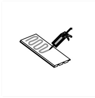
Image: Depiction of applying adhesive to the rear of a panel using a glue gun, illustrating the recommended serpentine pattern.
