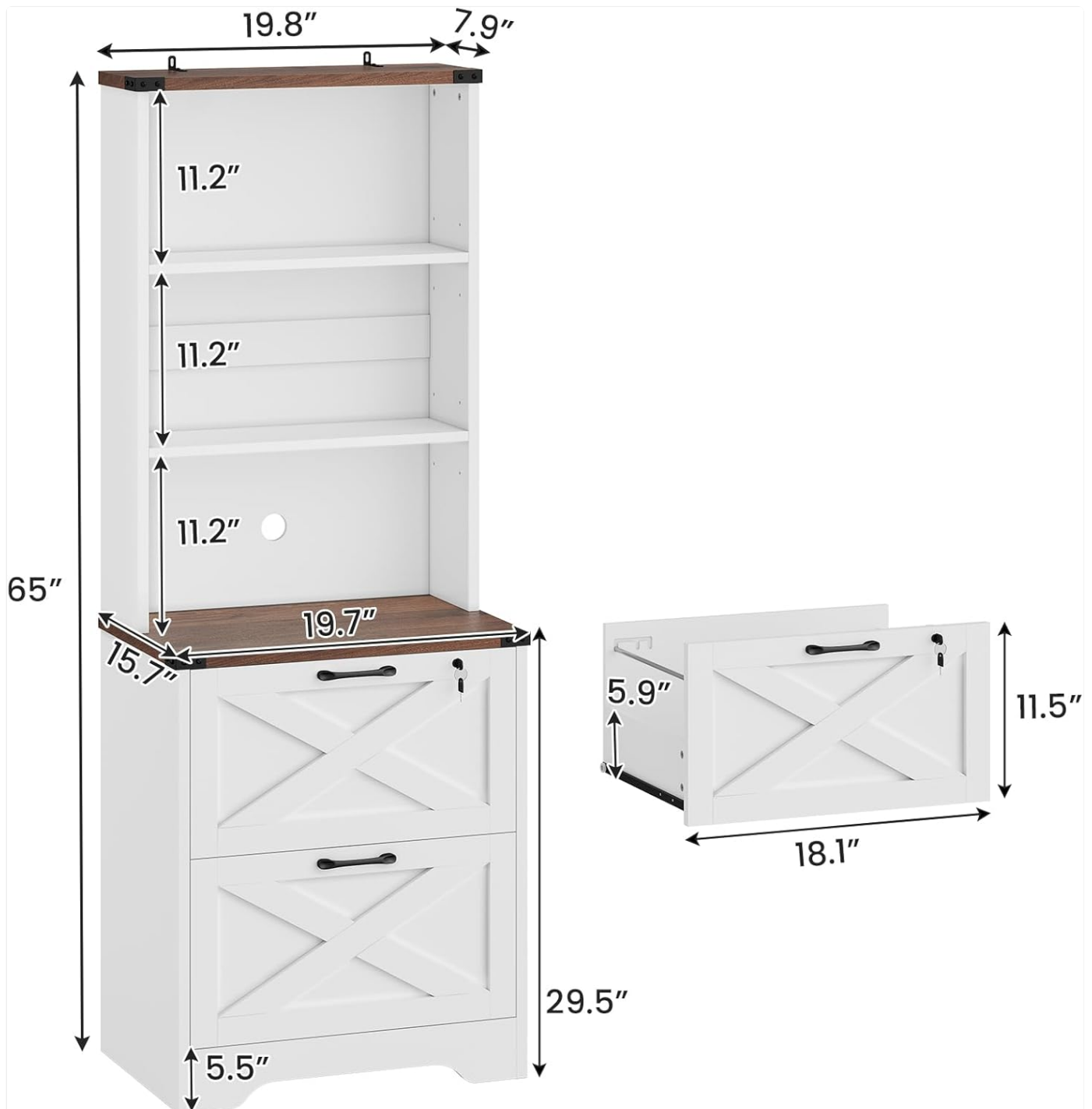
Image 4.1: Dimensional diagram of the file cabinet, showing overall height, width, depth, and internal shelf and drawer measurements.
