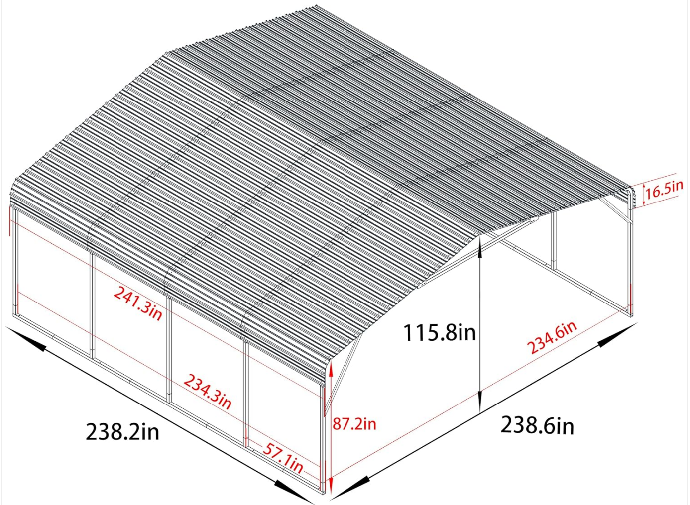
Figure 7.1: Carport Dimensions. This diagram provides a detailed overview of the carport's external and internal measurements, including the total storage area.
