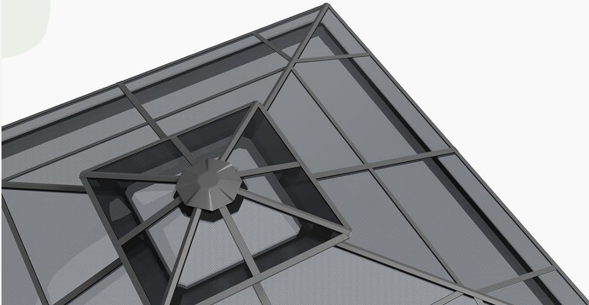
Figure 6: Double roof for ventilation and integrated water gutter system.
