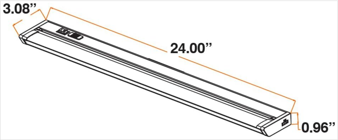
Figure 2: Product dimensions.
