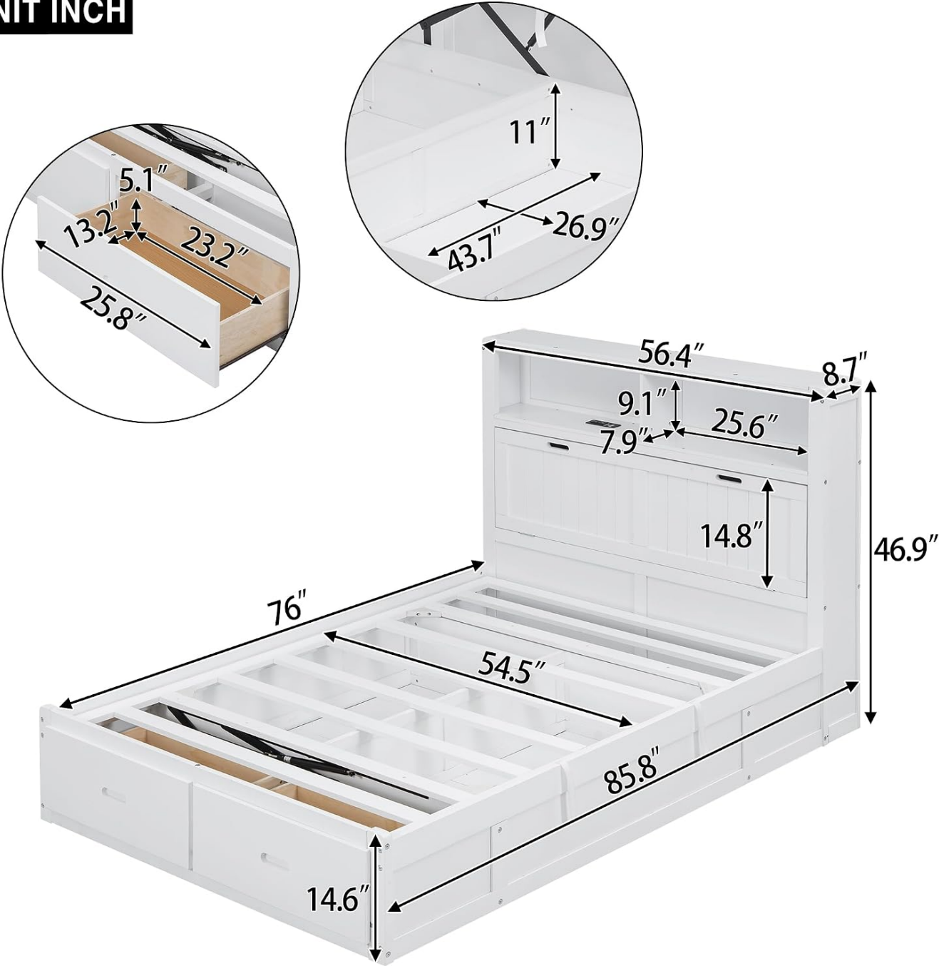
Figure 8.1: A technical diagram illustrating the precise dimensions of the LUMISOL Full White Platform Bed Frame, including length, width, height, and internal measurements of the headboard and storage compartments. All measurements are in inches.
