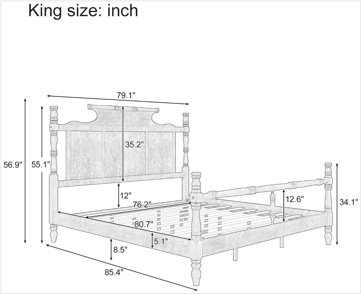
Image: Technical drawing illustrating the key dimensions of the King Size Platform Bed Frame in inches.
