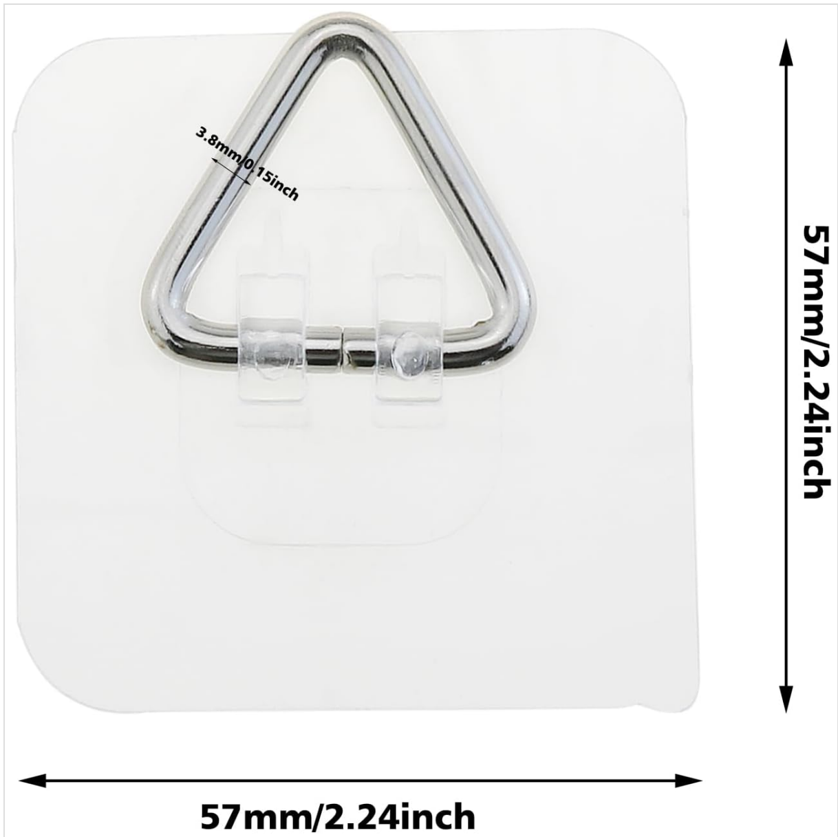
Figure 5: Detailed dimensions of a single ZHXSM adhesive hanger.
