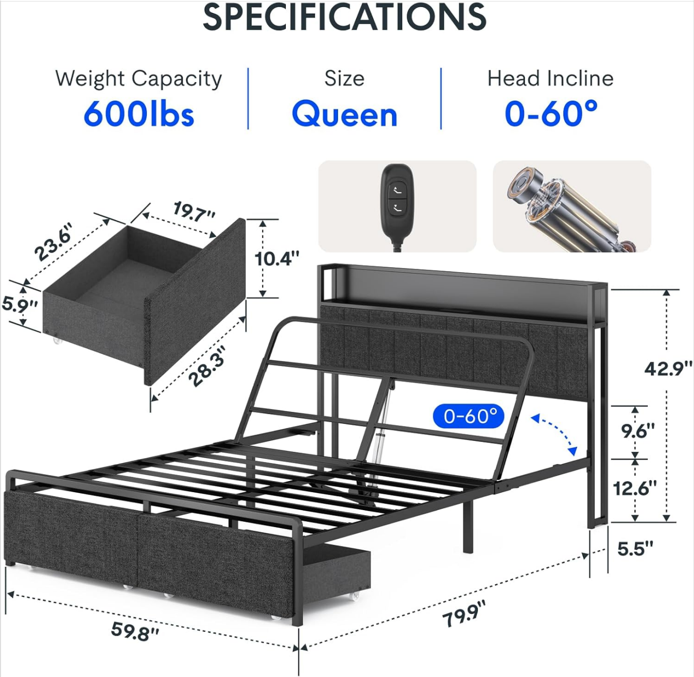
Figure 4.1: Product Dimensions and Key Components. This diagram illustrates the overall dimensions of the Queen size bed frame (79.9"L x 59.8"W x 42.9"H), the 0-60 degree head incline range, and the dimensions of the storage drawers (28.3"L x 19.7"W x 10.4"H).
