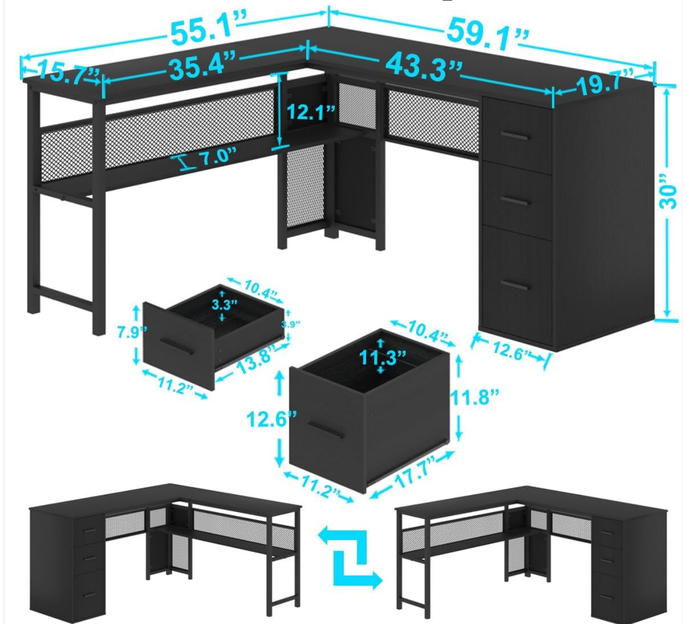
Image: Overview of desk dimensions, including the reversible L-shape and drawer sizes.
