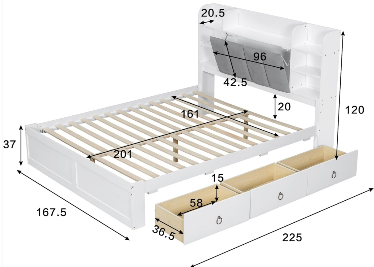
Image 4.1: Dimensional overview of the ModernLuxe Double Bed, indicating key measurements in centimeters.
