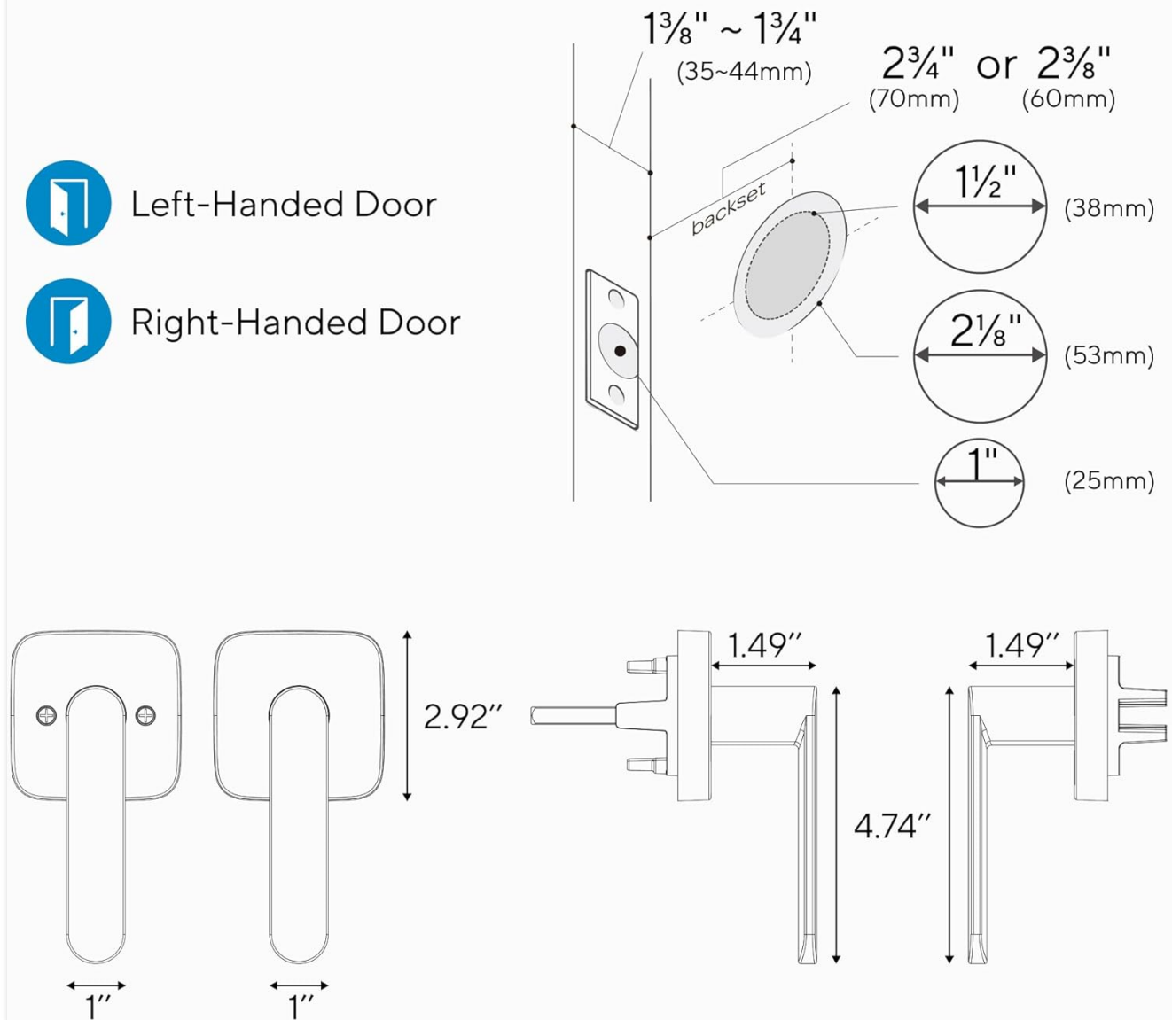
Figure 9: Door compatibility specifications, including recommended door thickness ( 1\frac{3}{8}" to 1\frac{3}{4}" ) and backset measurements for proper installation.
