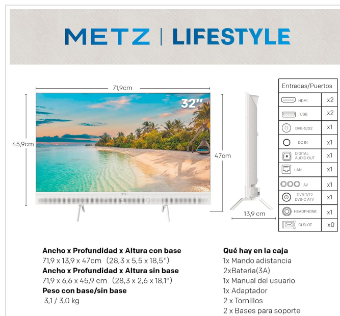
Image 2.1: Package contents and TV dimensions. The image displays the TV, remote, power cable, manual, bases, adapter, and screws. It also shows the TV's dimensions: 71.9 cm width, 47 cm height with base, 45.9 cm height without base, and 13.9 cm depth with base.
