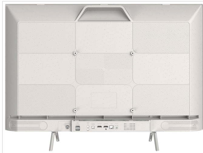
Image 3.2: Rear view of the Metz 32MTE7000Z TV, showing the arrangement of various input/output ports and the unique checkered back design.
