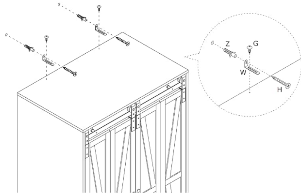
Figure 1: Anti-Tipping Device Installation. This diagram illustrates the correct method for securing the armoire to the wall using the provided anti-tipping hardware, ensuring stability and preventing accidental falls.
